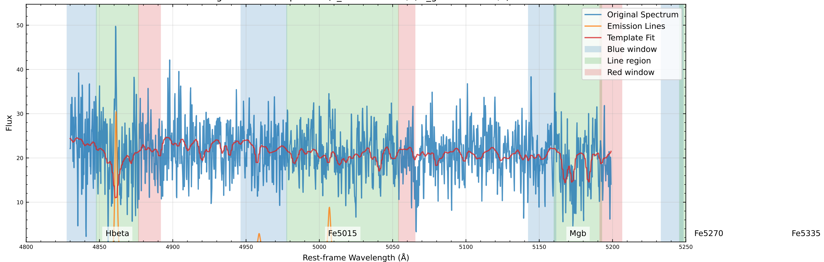
Original Data Comparison (v_star=35.5 km/s, v_gas=-14.8 km/s)
