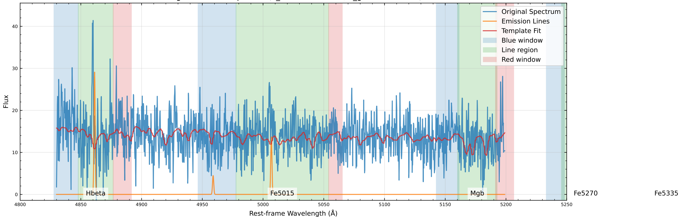
Original Data Comparison (v_star=-93.6 km/s, v_gas=-98.9 km/s)
