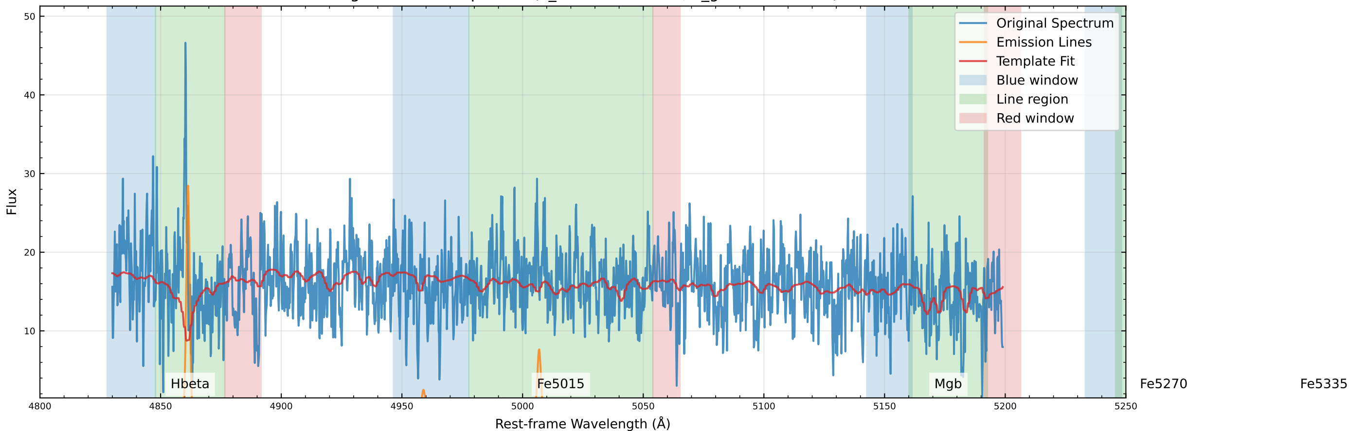
Original Data Comparison (v_star=-58.5 km/s, v_gas=-64.5 km/s)
