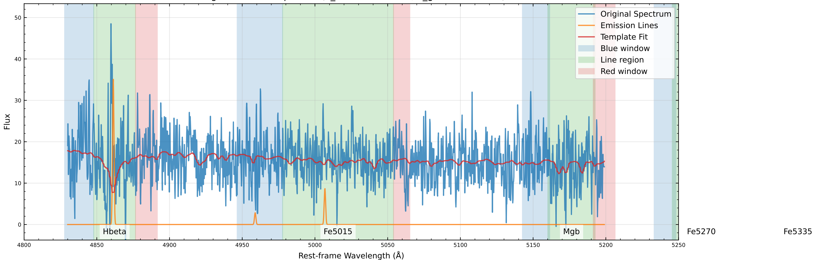
Original Data Comparison (v_star=-58.2 km/s, v_gas=-77.0 km/s)
