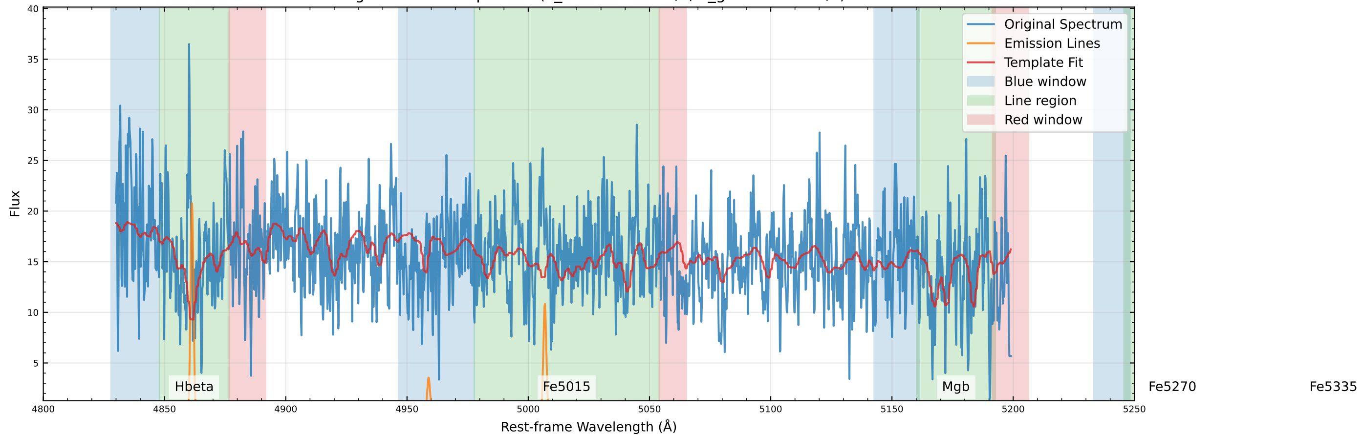
Original Data Comparison (v_star=-71.0 km/s, v_gas=-71.6 km/s)
