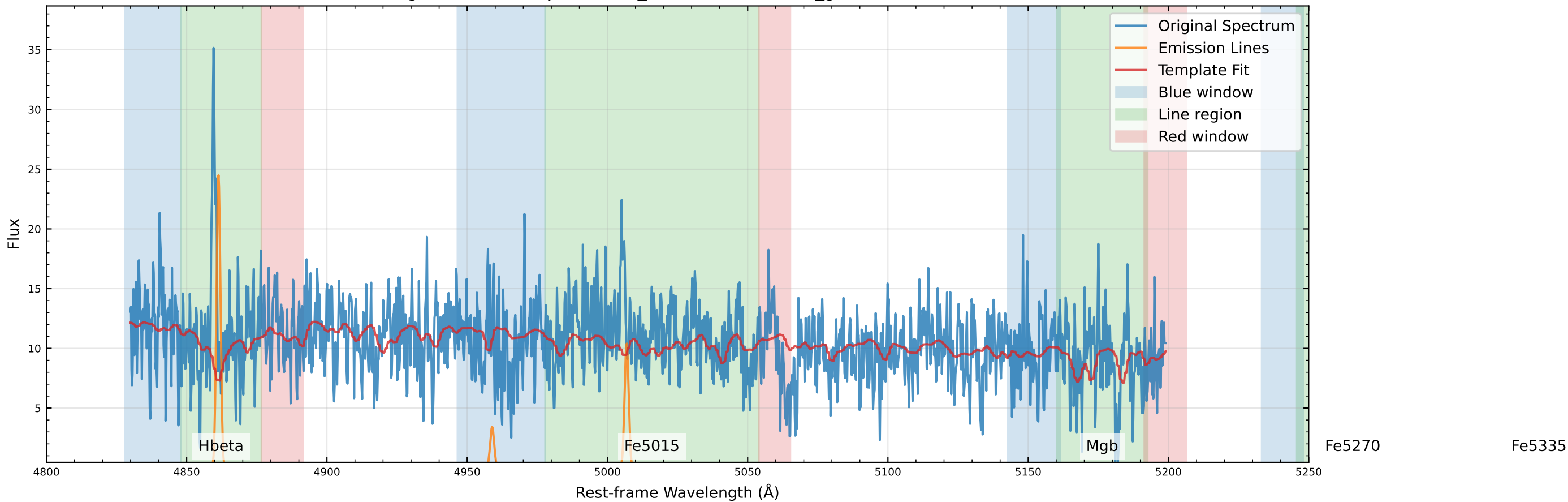
Original Data Comparison (v_star=-96.4 km/s, v_gas=-99.0 km/s)
