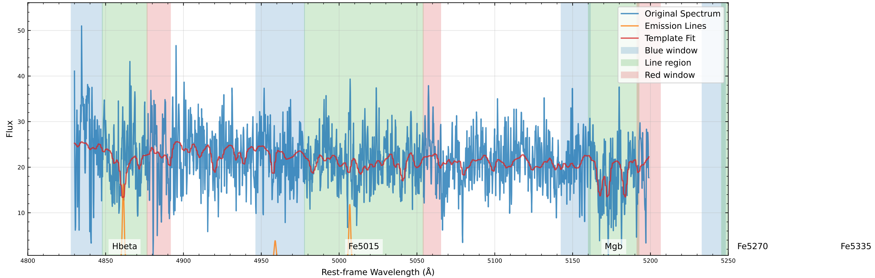
Original Data Comparison (v_star=-29.3 km/s, v_gas=-19.4 km/s)
