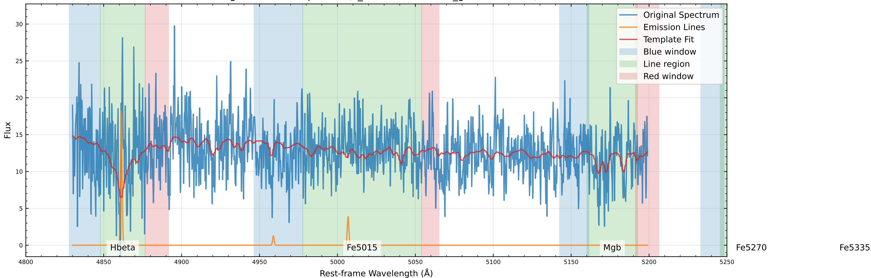
Original Data Comparison (v_star=26.2 km/s, v_gas=40.2 km/s)
