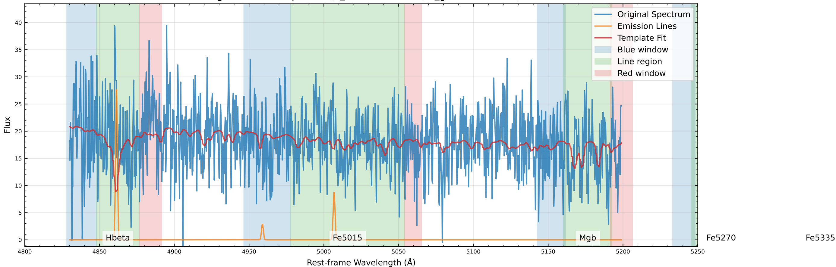
Original Data Comparison (v_star=-77.3 km/s, v_gas=-55.0 km/s)
