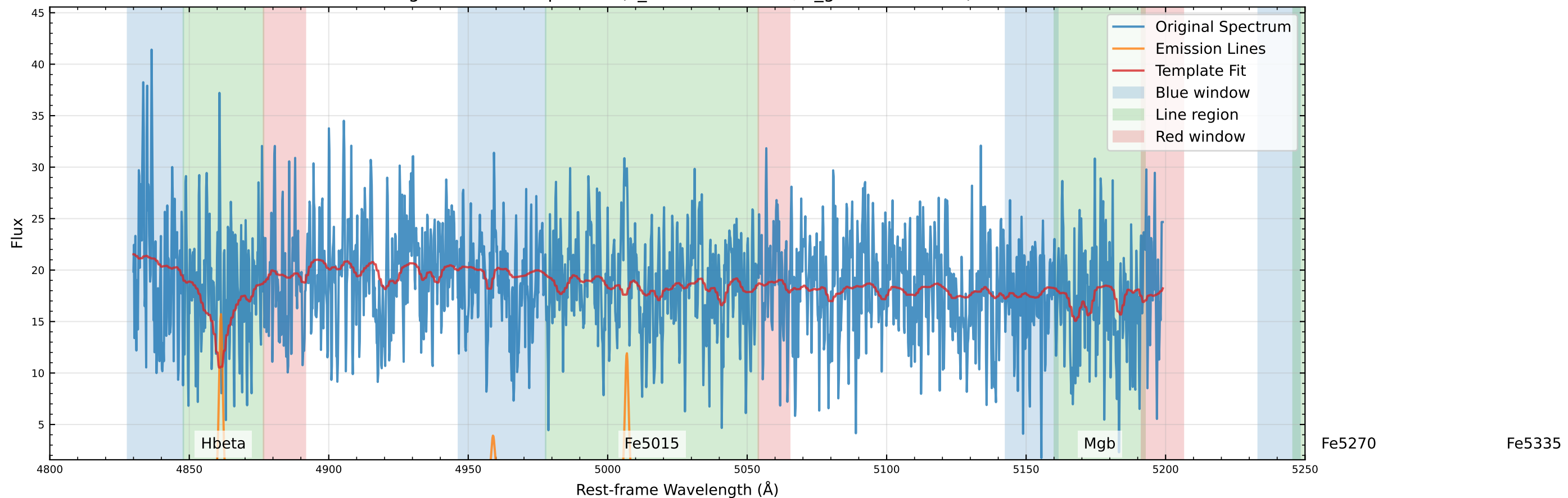
Original Data Comparison (v_star=-47.7 km/s, v_gas=-40.8 km/s)
