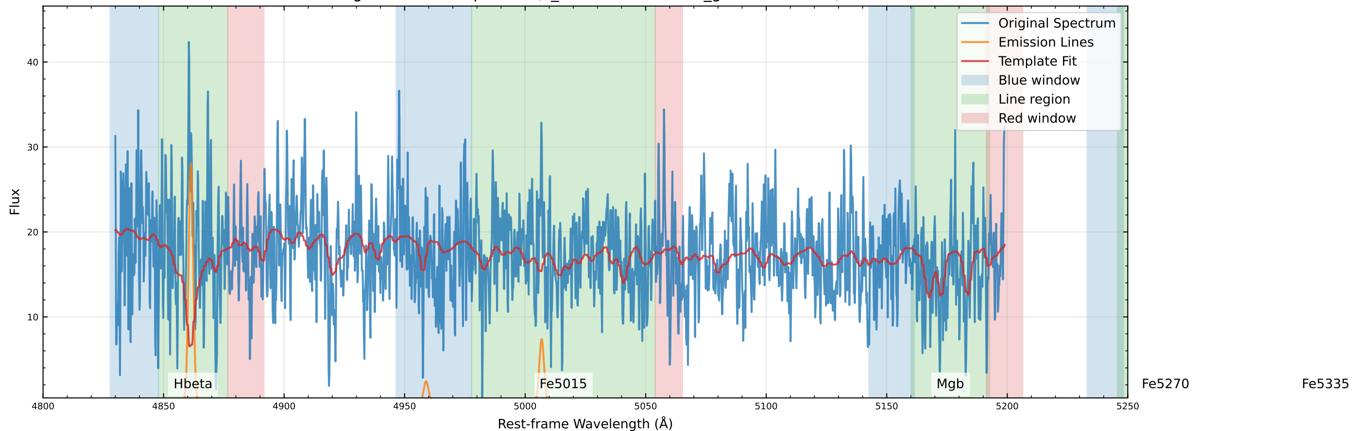
Original Data Comparison (v_star=-27.8 km/s, v_gas=-28.5 km/s)
