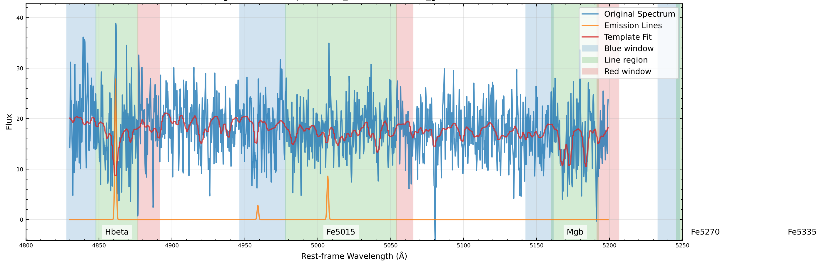
Original Data Comparison (v_star=9.1 km/s, v_gas=9.5 km/s)
