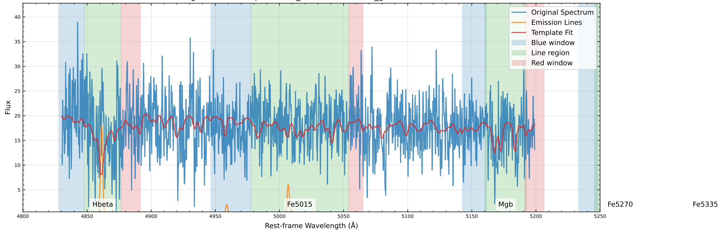
Original Data Comparison (v_star=75.8 km/s, v_gas=47.6 km/s)
