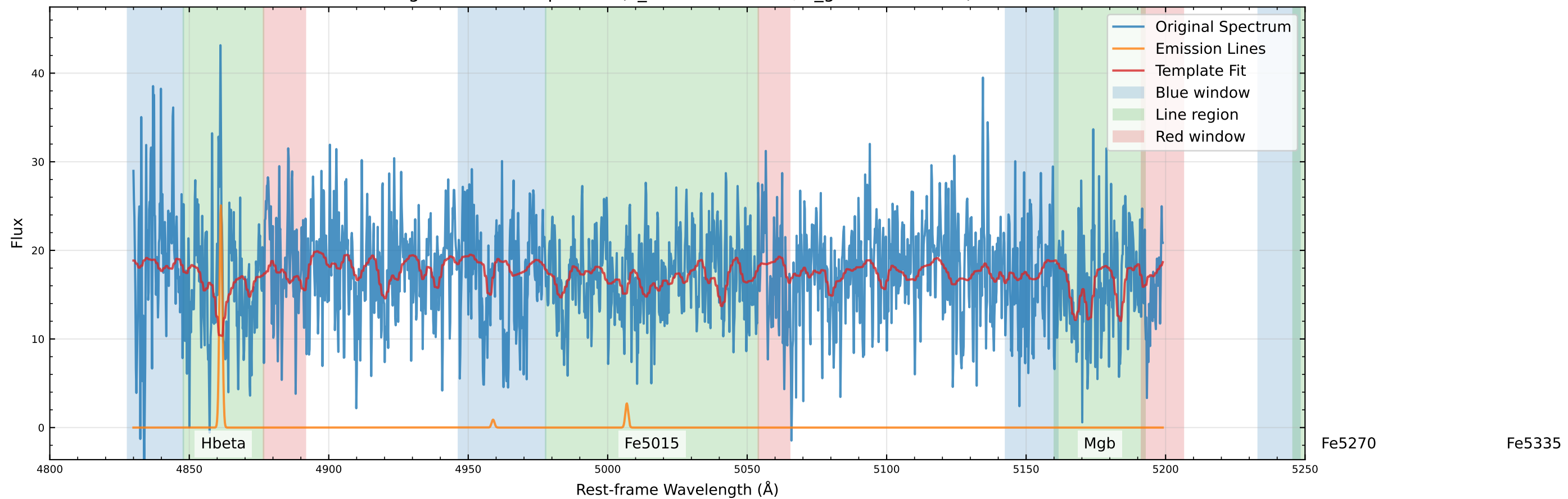
Original Data Comparison (v_star=-24.1 km/s, v_gas=-17.9 km/s)
