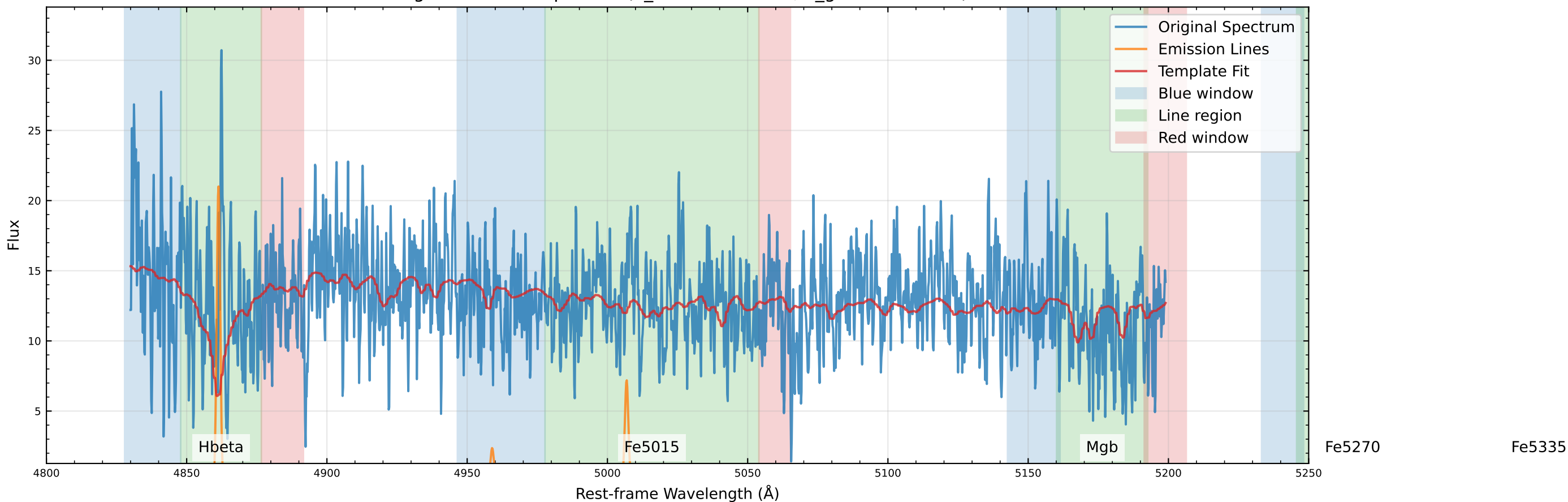
Original Data Comparison (v_star=85.9 km/s, v_gas=69.9 km/s)
