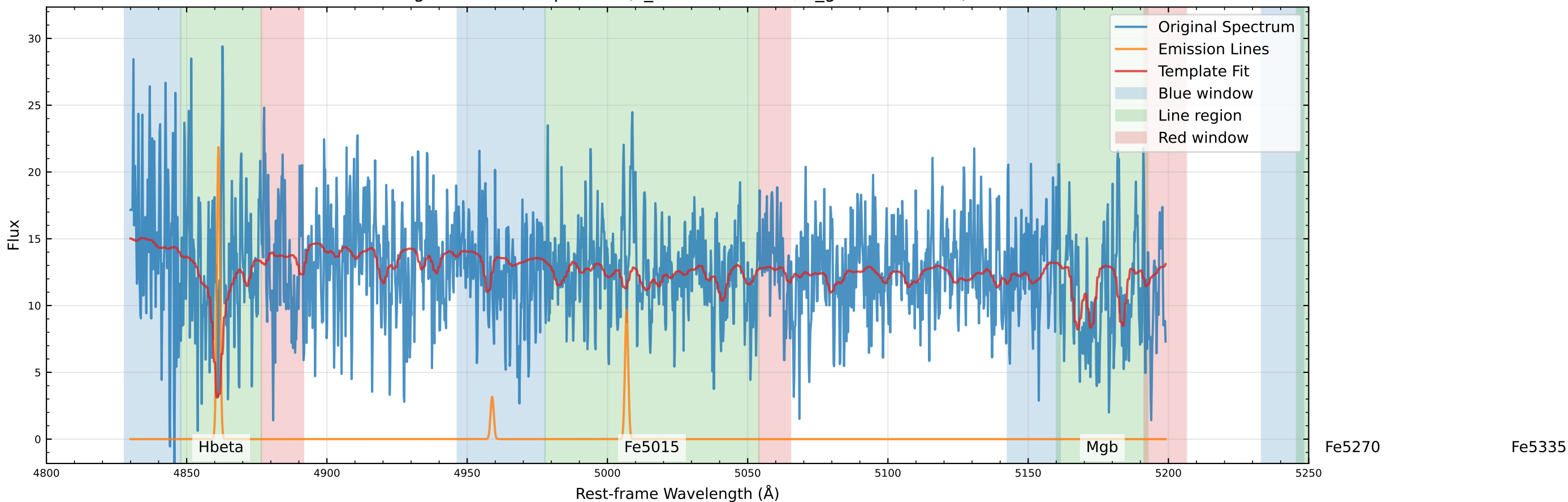
Original Data Comparison (v_star=94.1 km/s, v_gas=91.4 km/s)
