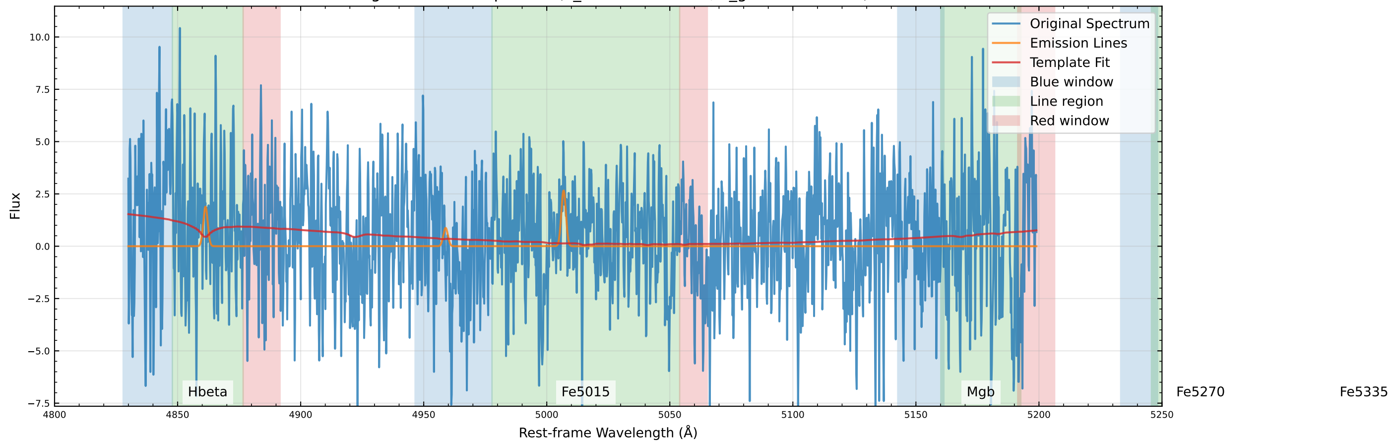
Original Data Comparison (v_star=-14.8 km/s, v_gas=-28.7 km/s)
