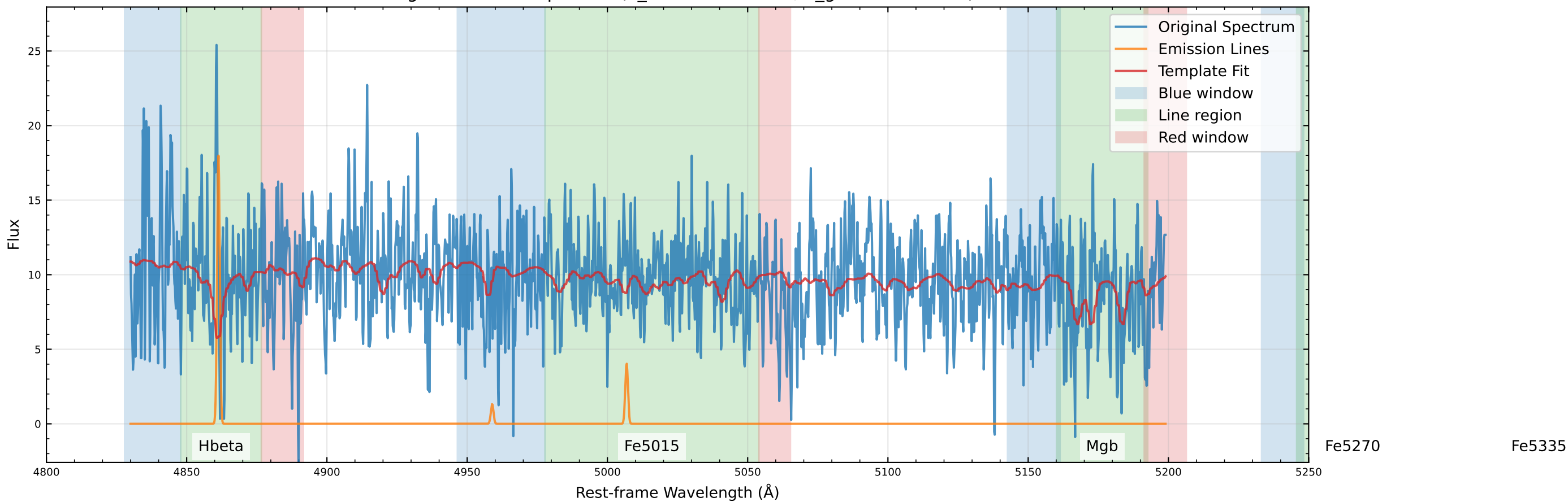
Original Data Comparison (v_star=-74.1 km/s, v_gas=-50.3 km/s)
