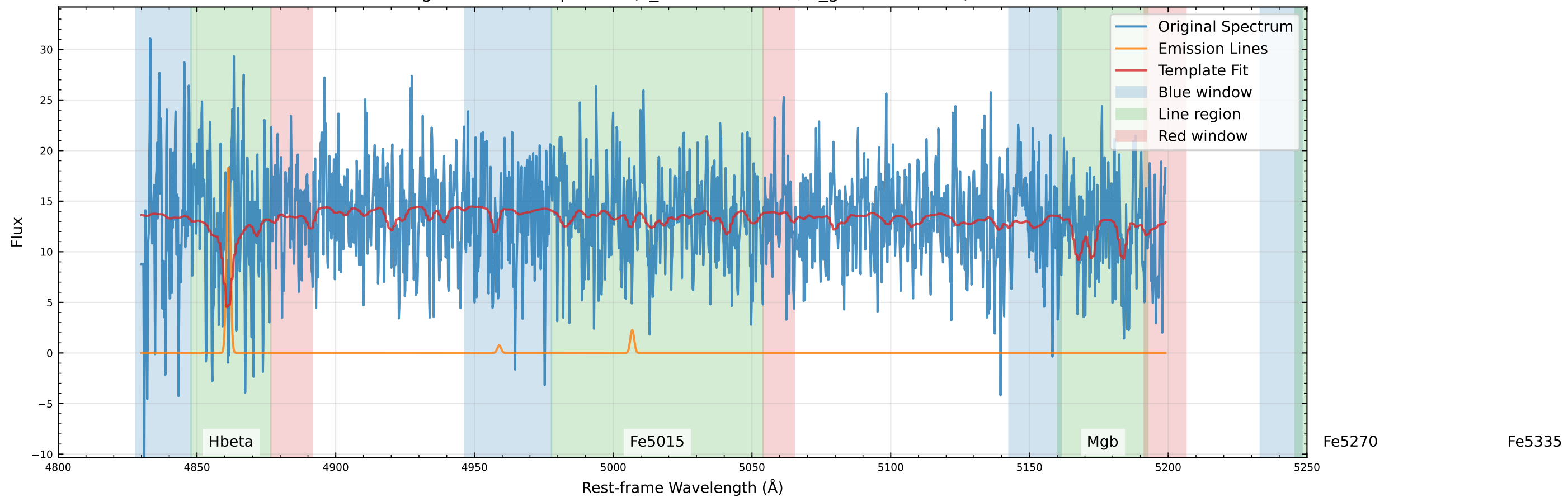
Original Data Comparison (v_star=89.4 km/s, v_gas=91.2 km/s)
