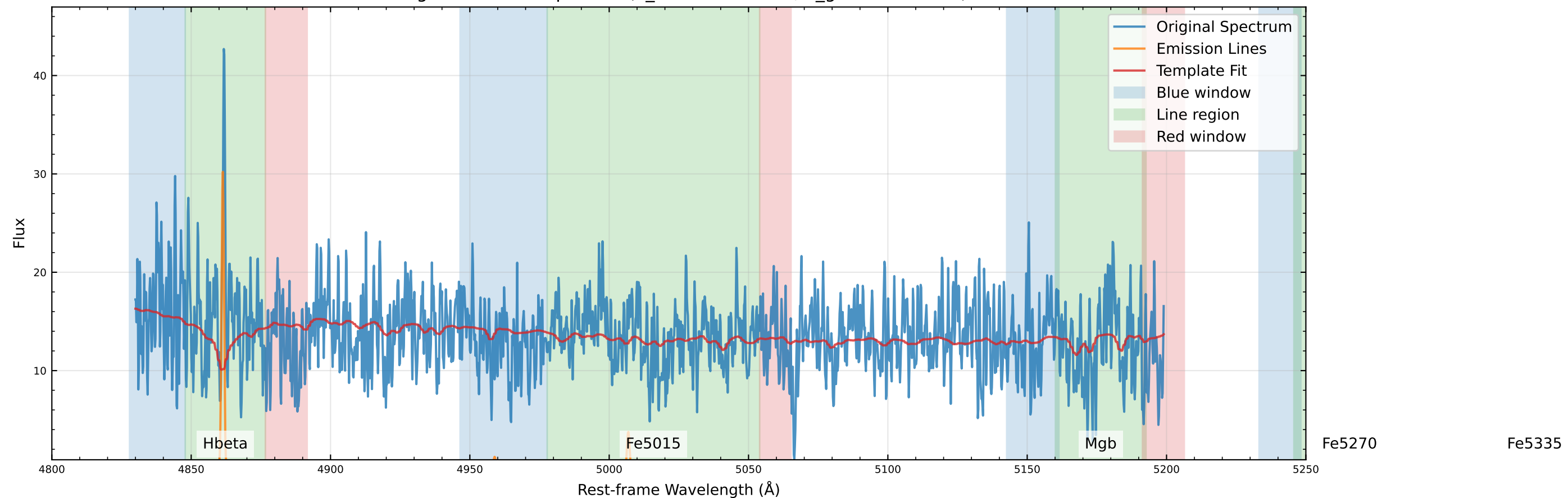
Original Data Comparison (v_star=44.4 km/s, v_gas=27.5 km/s)
