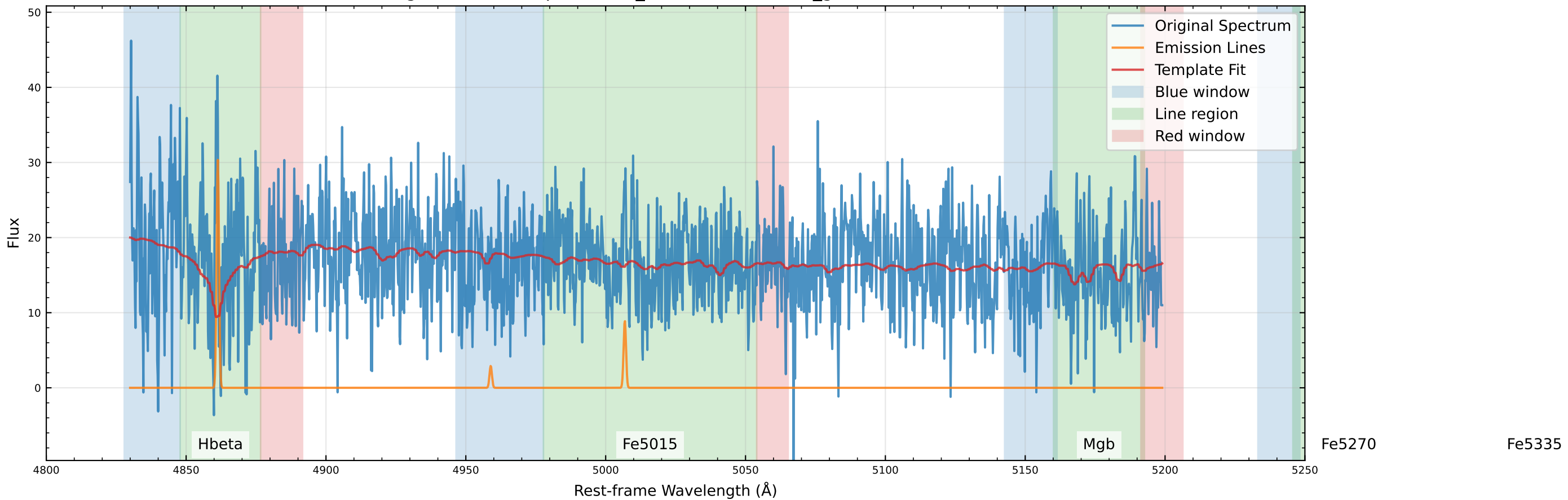
Original Data Comparison (v_star=-42.1 km/s, v_gas=-23.6 km/s)
