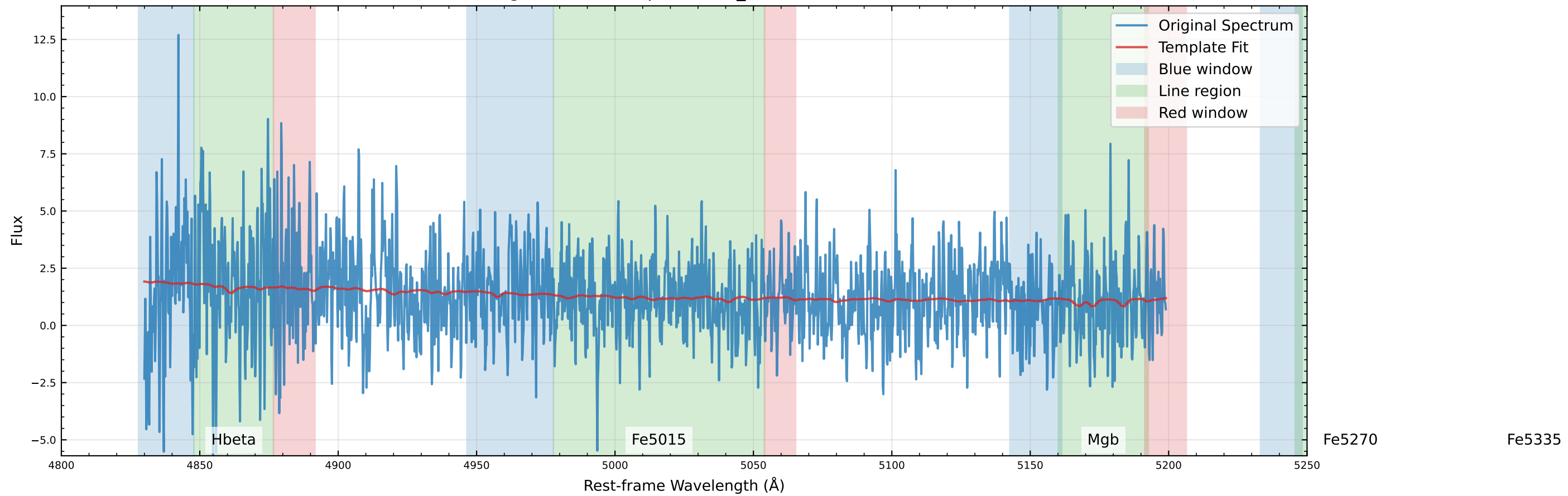
Original Data Comparison ( v_{\text{star}}=-9.1 km/s)
