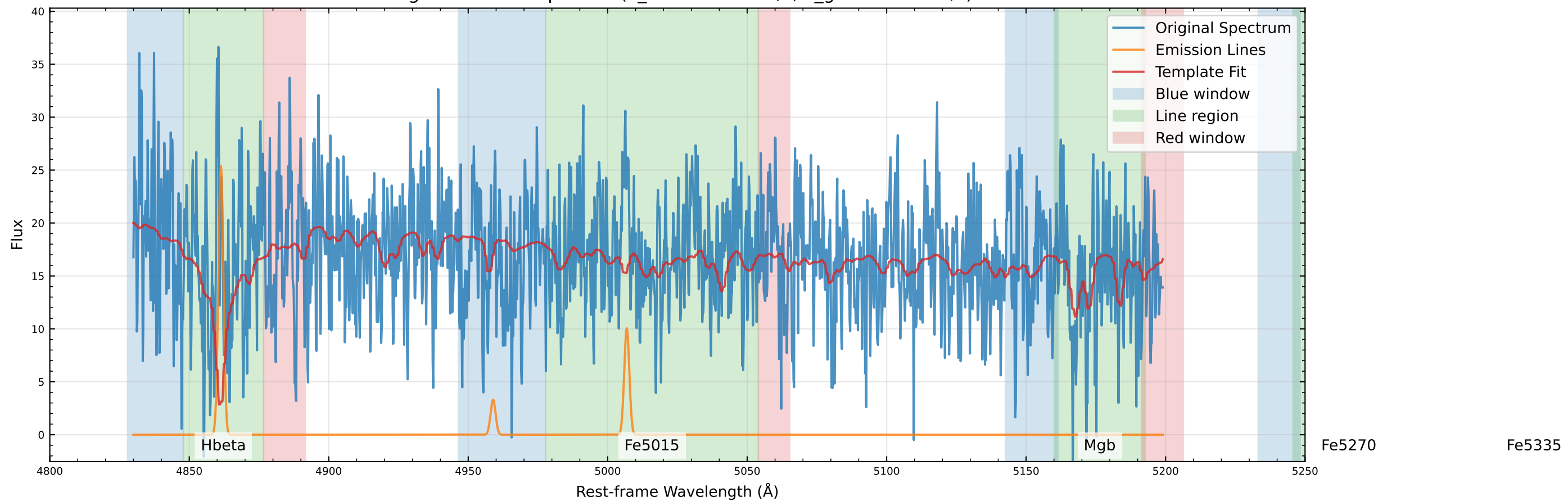
Original Data Comparison (v_star=-64.5 km/s, v_gas=-53.8 km/s)
