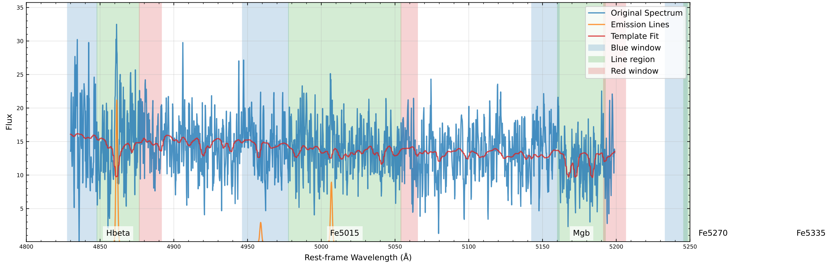
Original Data Comparison (v_star=-32.8 km/s, v_gas=-26.3 km/s)
