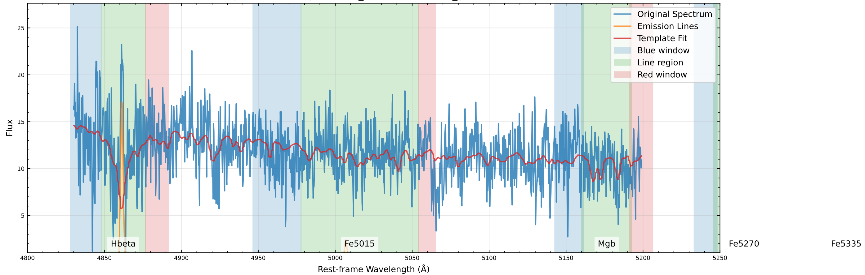
Original Data Comparison (v_star=10.7 km/s, v_gas=1.8 km/s)
