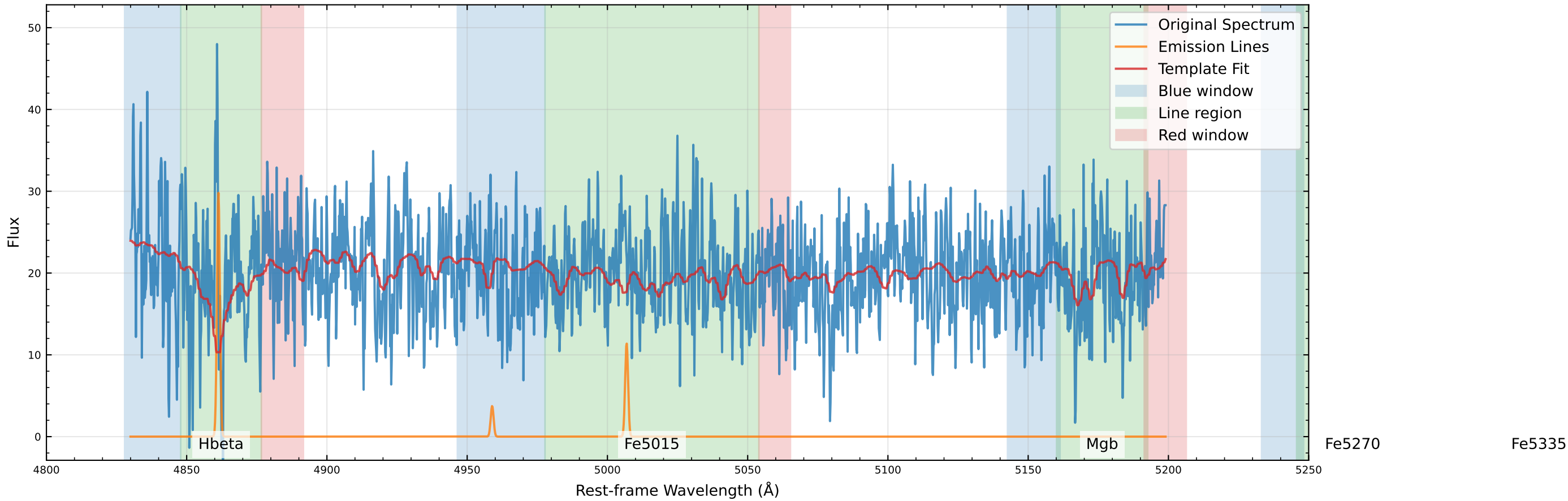
Original Data Comparison (v_star=-51.9 km/s, v_gas=-46.5 km/s)
