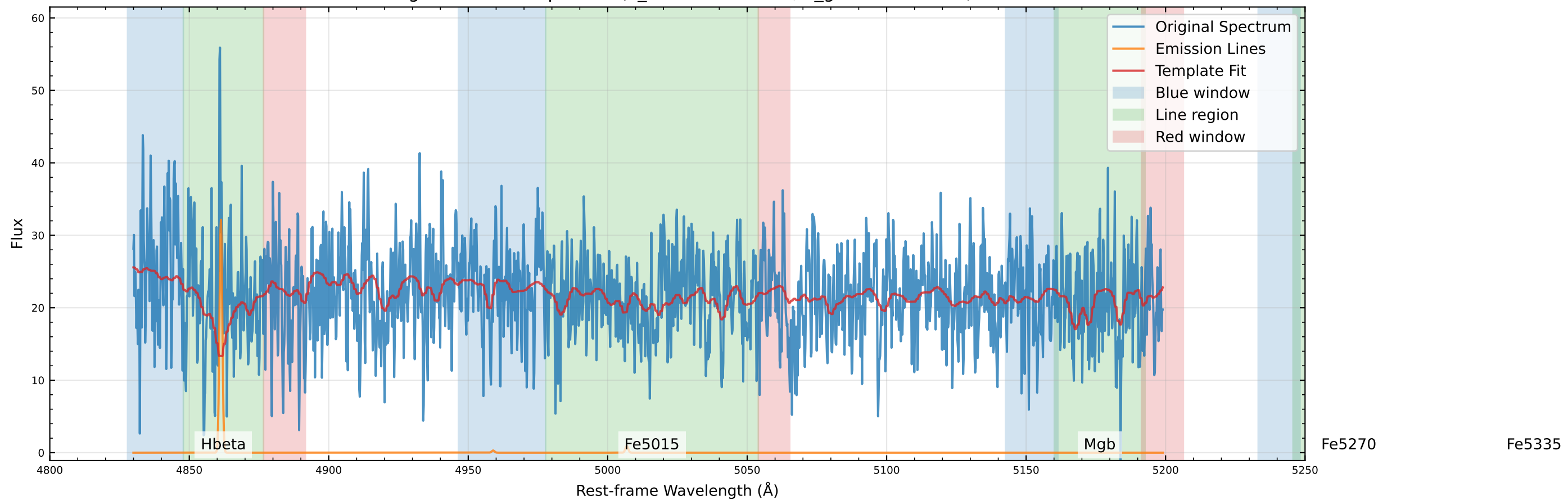
Original Data Comparison (v_star=-23.5 km/s, v_gas=-13.6 km/s)
