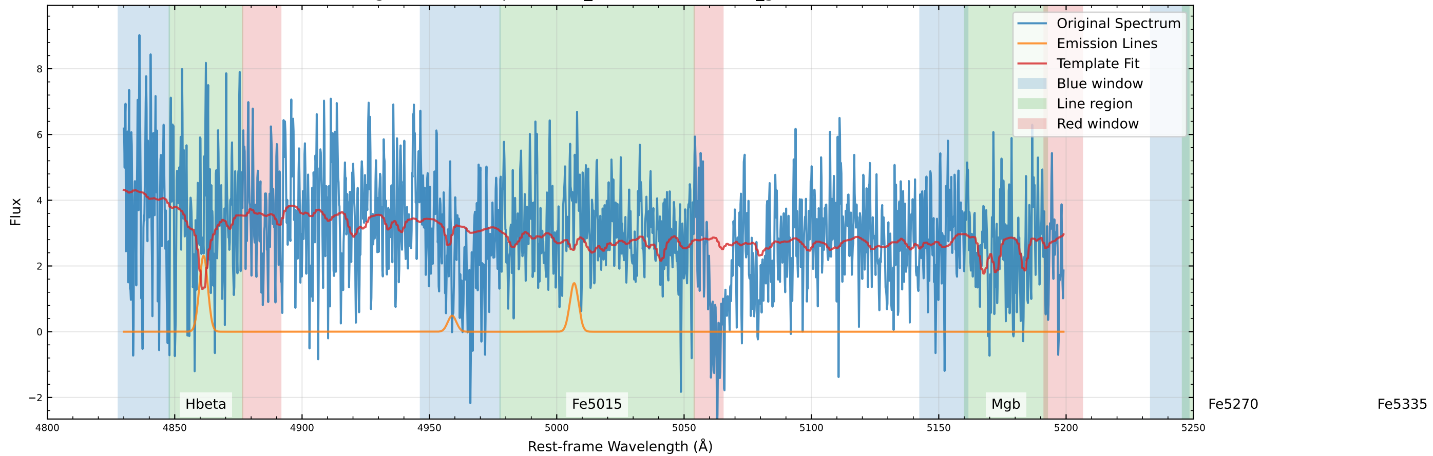
Original Data Comparison (v_star=-101.5 km/s, v_gas=-1.5 km/s)
