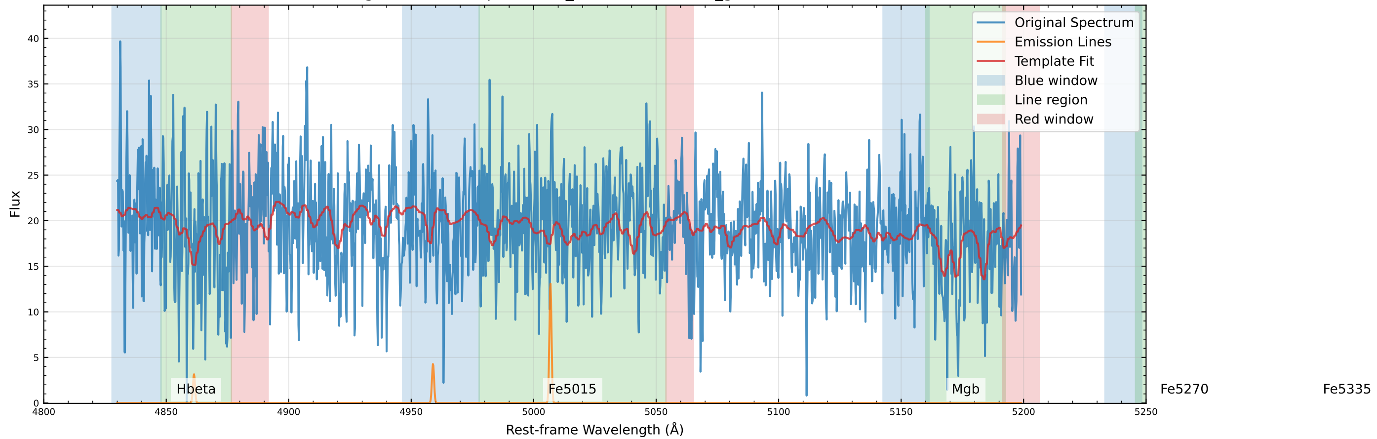
Original Data Comparison (v_star=28.1 km/s, v_gas=33.3 km/s)
