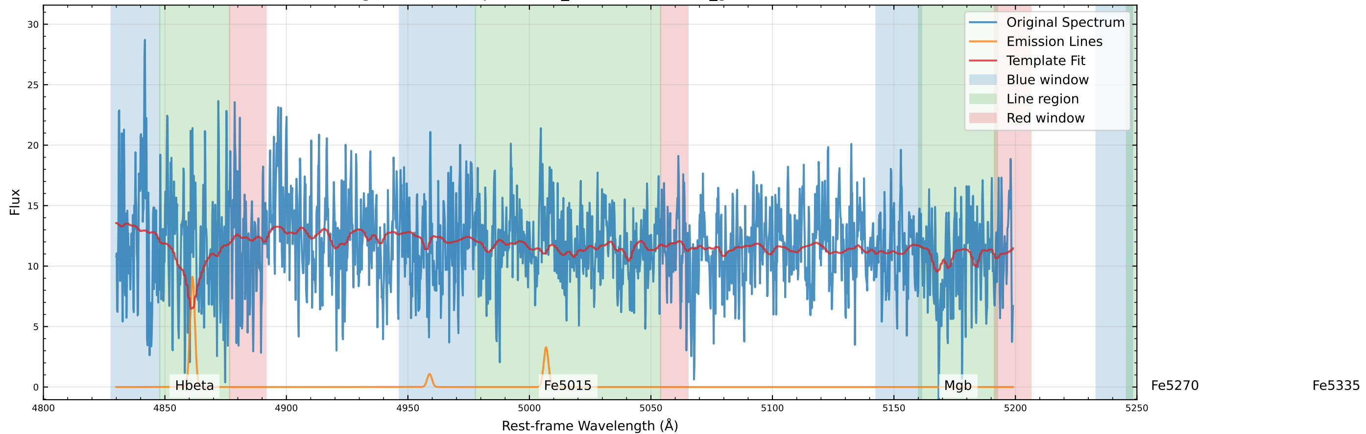
Original Data Comparison (v_star=39.3 km/s, v_gas=24.5 km/s)
