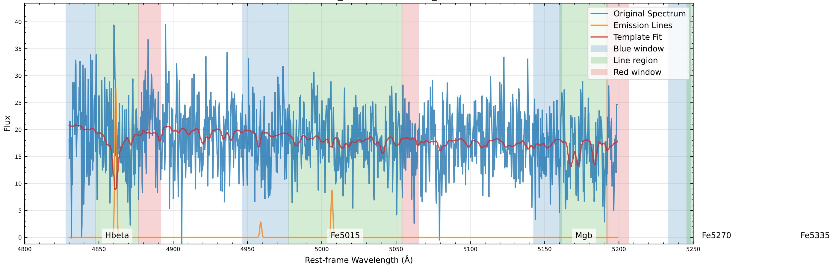
Original Data Comparison (v_star=-77.3 km/s, v_gas=-55.0 km/s)
