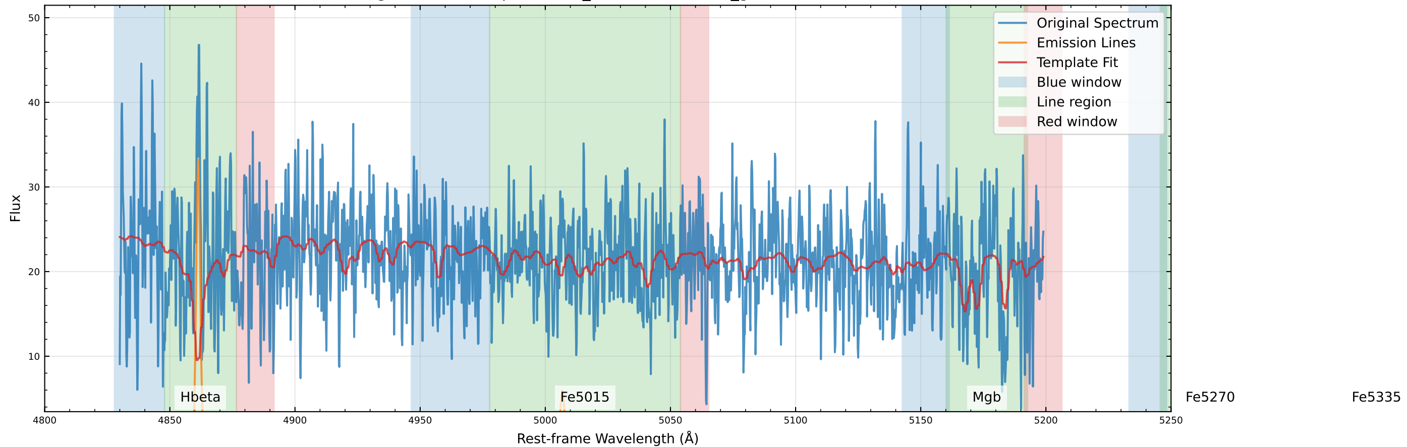
Original Data Comparison (v_star=-4.6 km/s, v_gas=-5.5 km/s)
