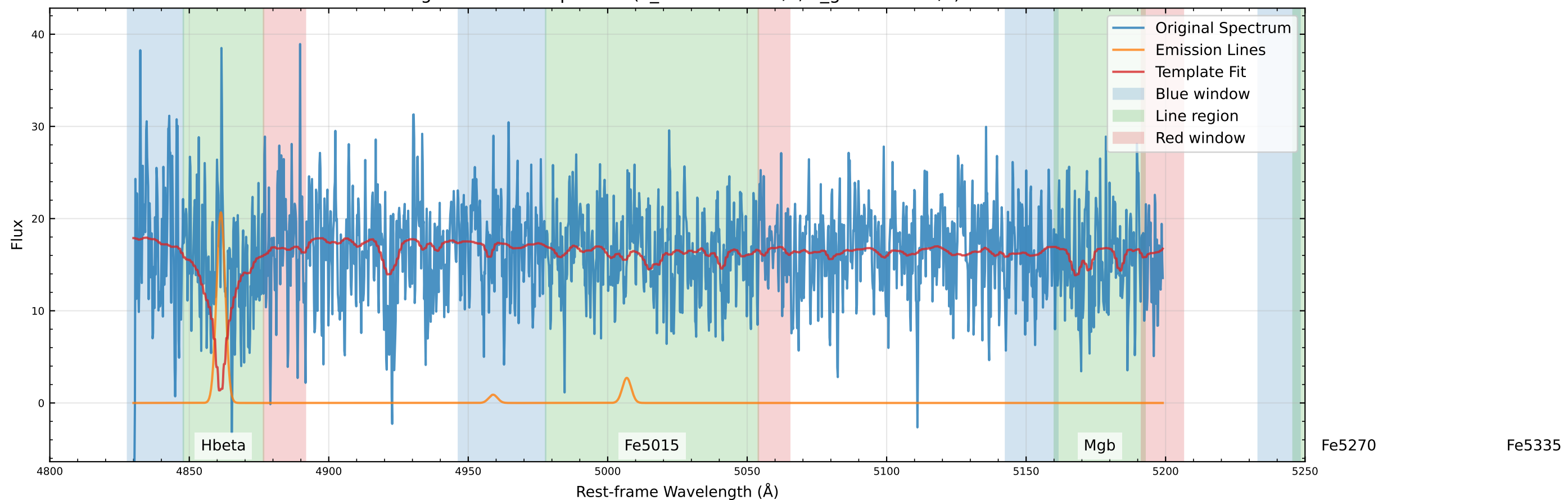
Original Data Comparison (v_star=43.2 km/s, v_gas=8.4 km/s)
