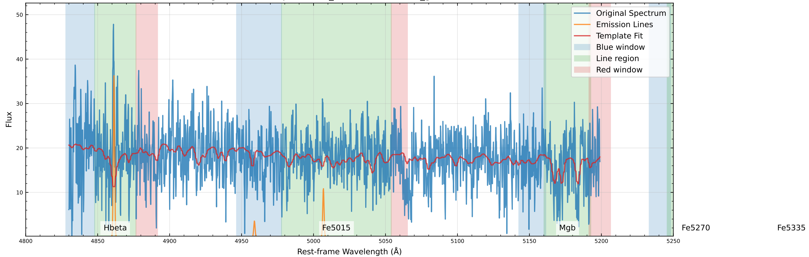
Original Data Comparison (v_star=-17.5 km/s, v_gas=-23.5 km/s)
