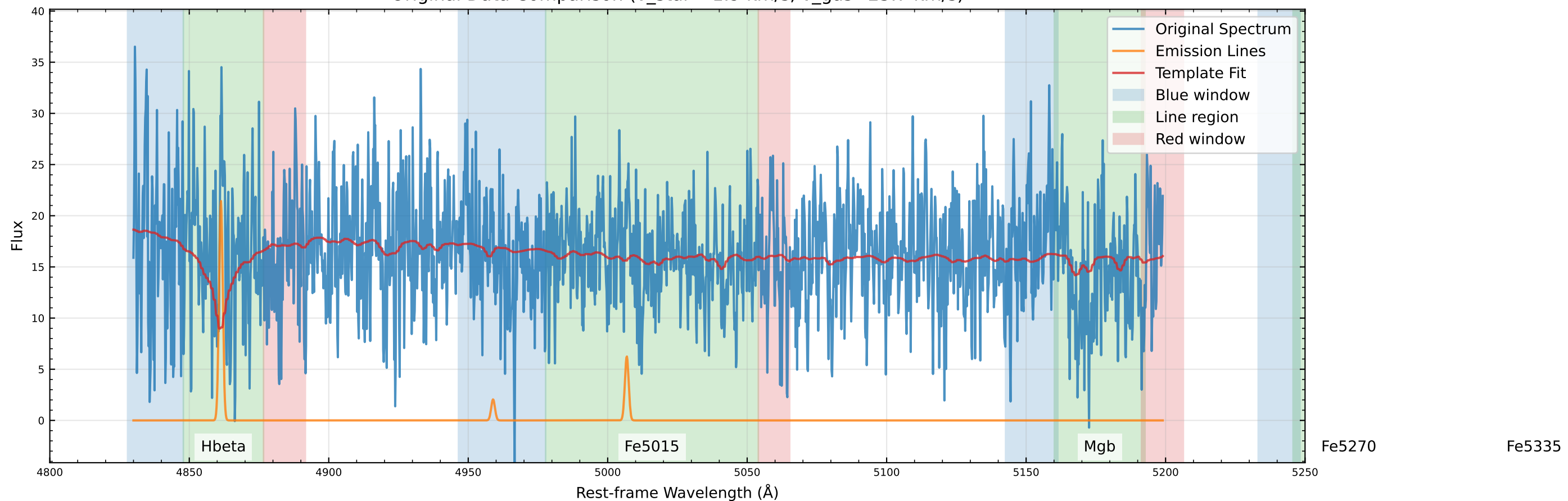
Original Data Comparison (v_star=-1.9 km/s, v_gas=23.7 km/s)
