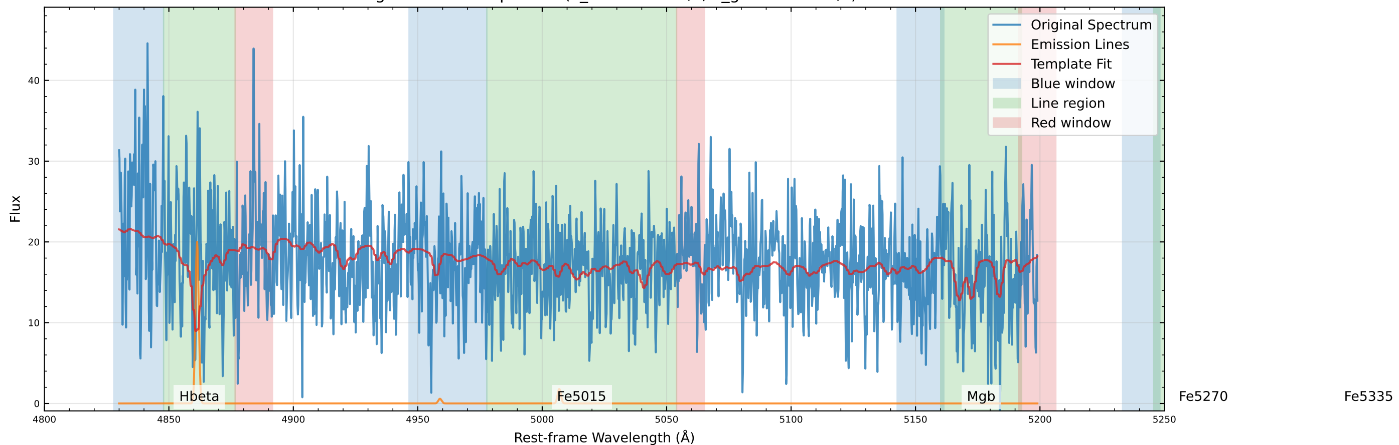
Original Data Comparison (v_star=1.8 km/s, v_gas=27.1 km/s)
