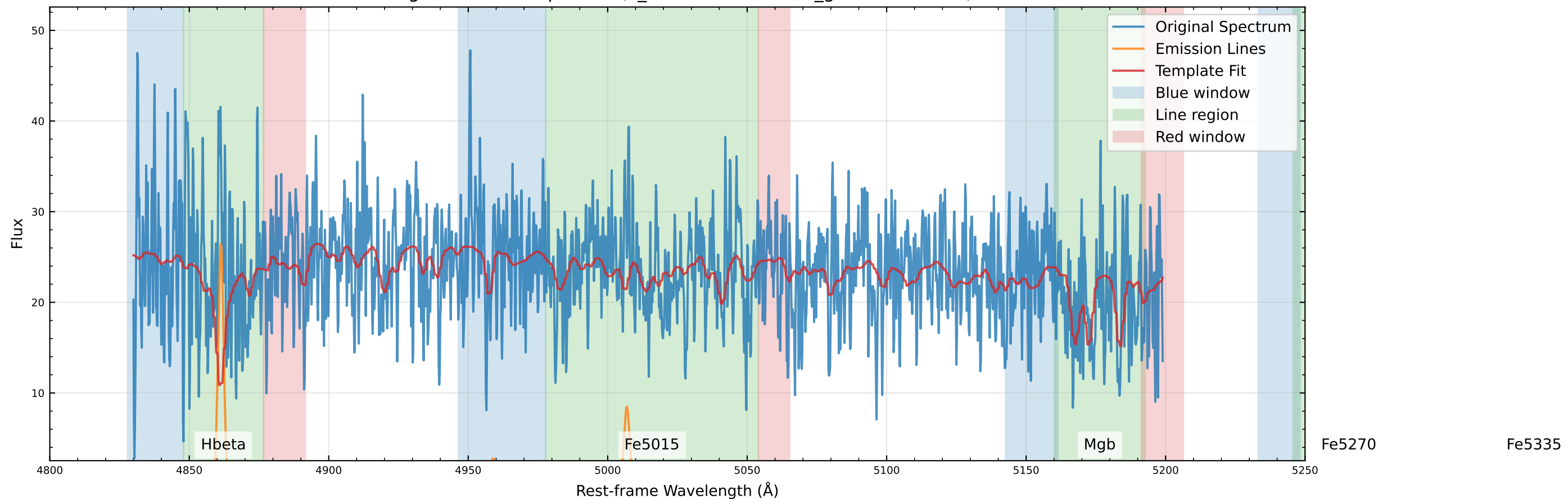
Original Data Comparison (v_star=-13.6 km/s, v_gas=-13.8 km/s)
