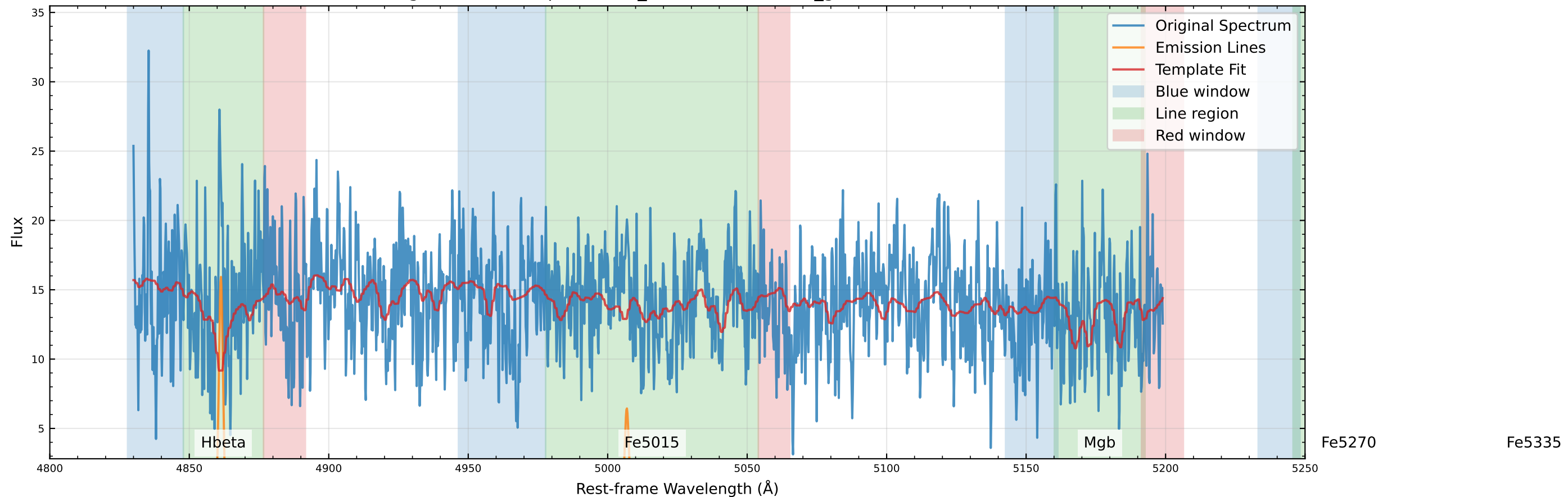
Original Data Comparison (v_star=-30.8 km/s, v_gas=-14.6 km/s)
