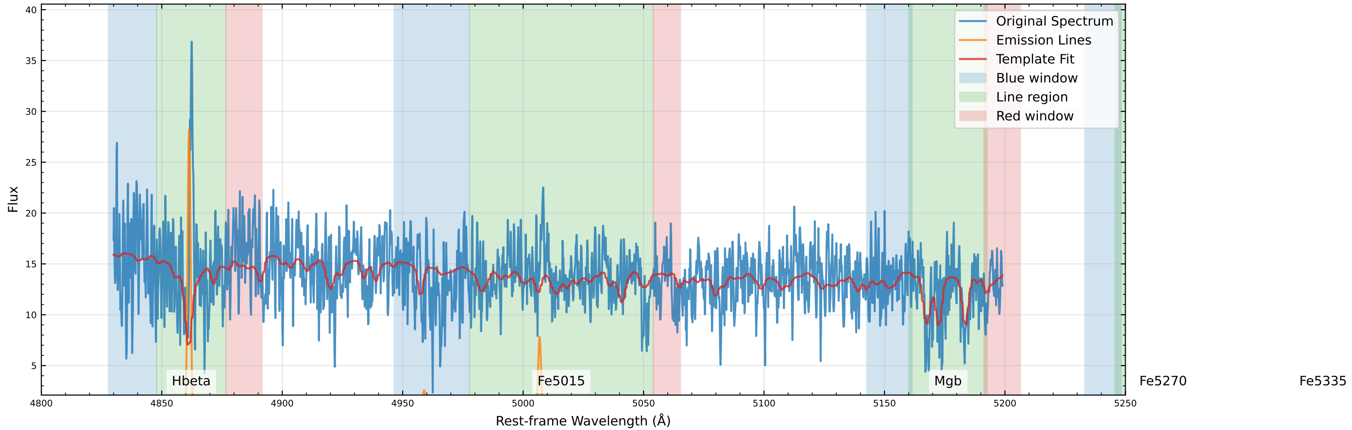
Original Data Comparison (v_star=34.5 km/s, v_gas=58.4 km/s)
