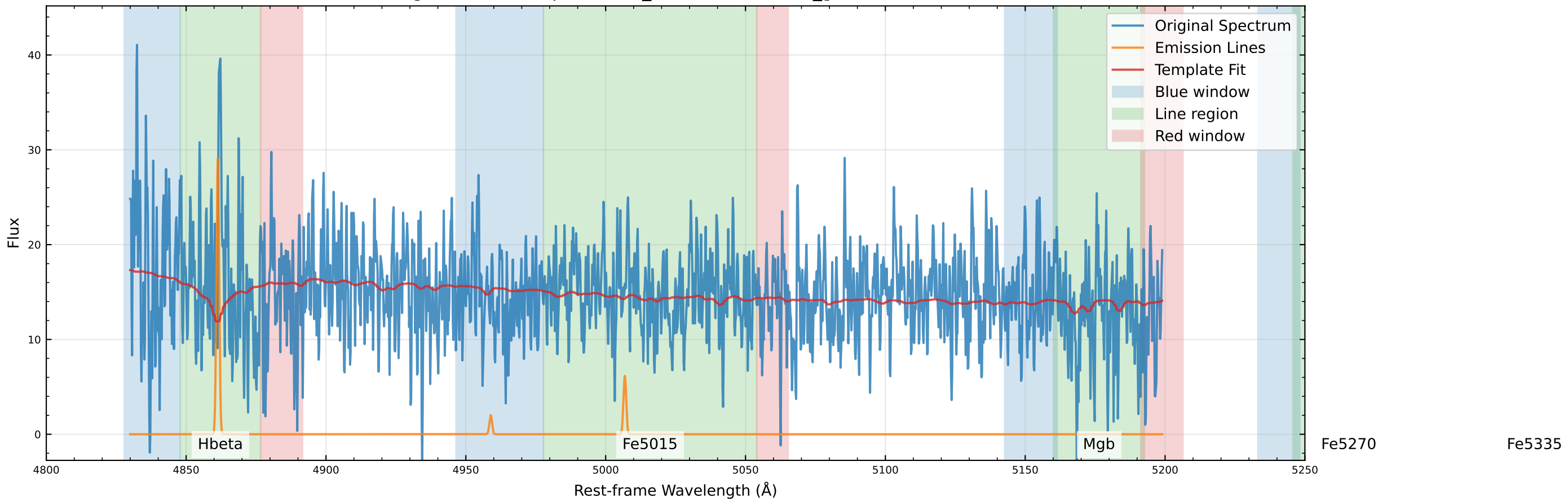
Original Data Comparison (v_star=34.0 km/s, v_gas=47.6 km/s)
