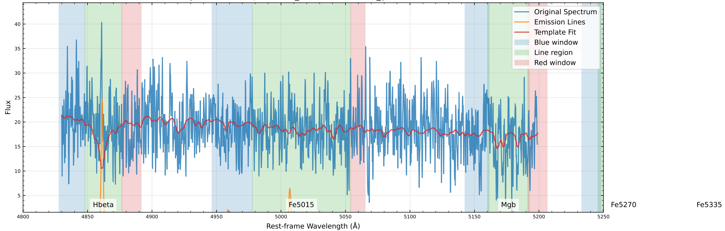
Original Data Comparison (v_star=-12.4 km/s, v_gas=-36.5 km/s)
