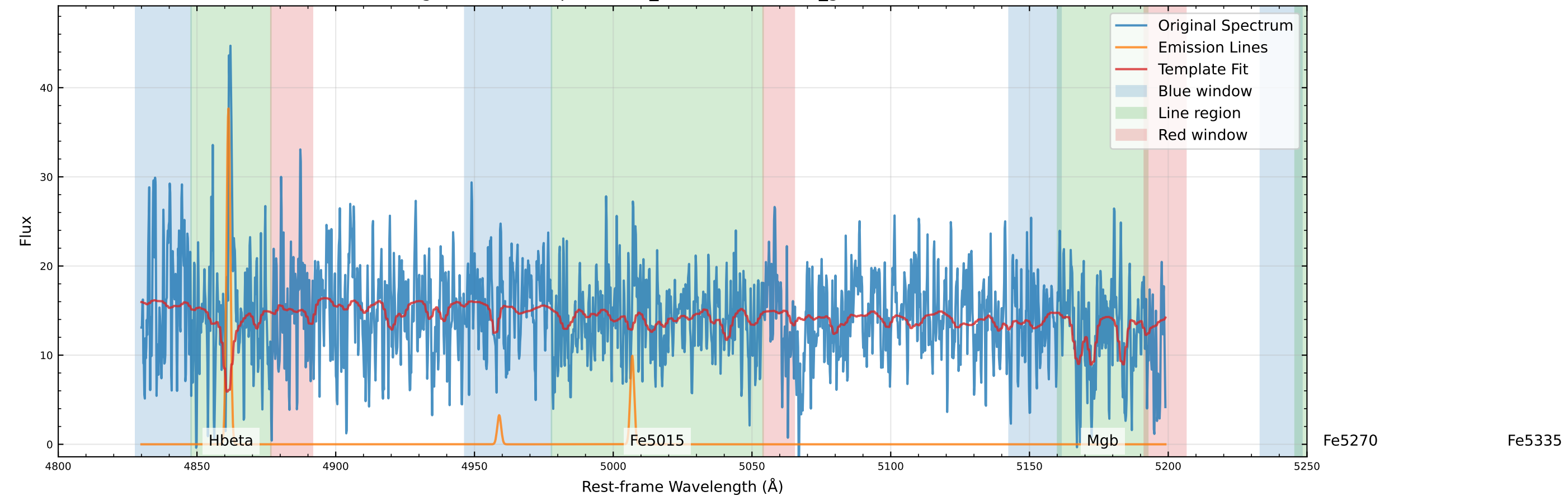
Original Data Comparison (v_star=36.7 km/s, v_gas=41.2 km/s)
