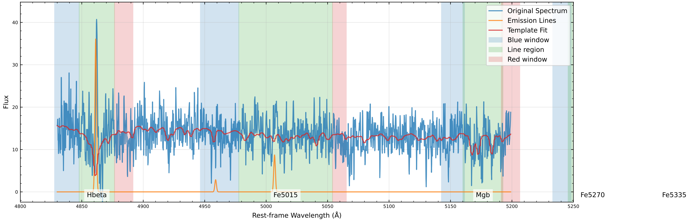
Original Data Comparison (v_star=52.5 km/s, v_gas=46.9 km/s)
