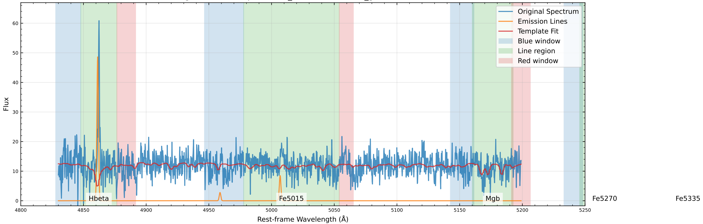
Original Data Comparison (v_star=54.2 km/s, v_gas=58.5 km/s)
