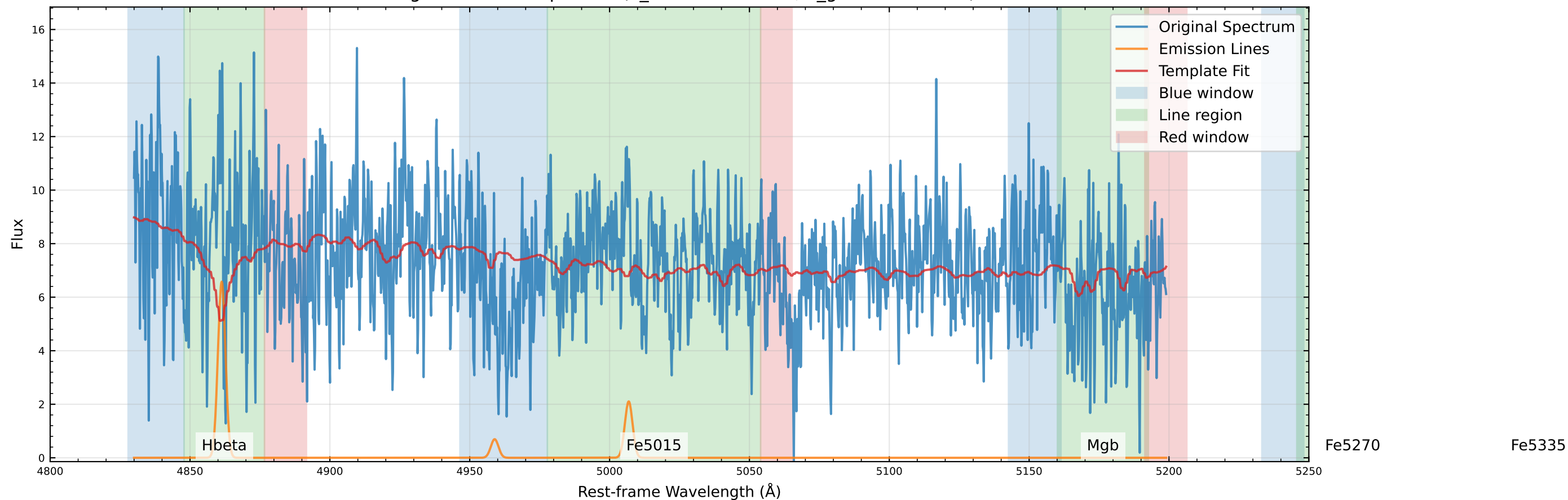
Original Data Comparison (v_star=-88.5 km/s, v_gas=-74.2 km/s)
