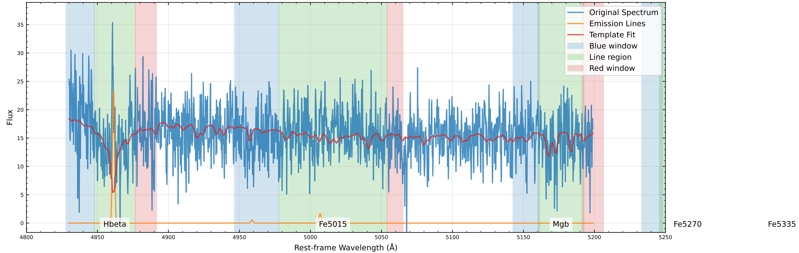
Original Data Comparison (v_star=-28.8 km/s, v_gas=-33.2 km/s)
