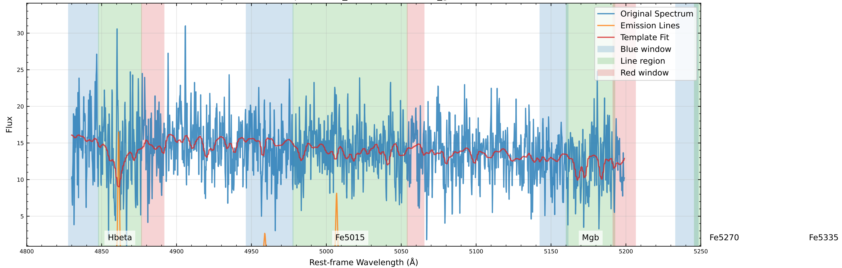
Original Data Comparison (v_star=-53.8 km/s, v_gas=-53.9 km/s)
