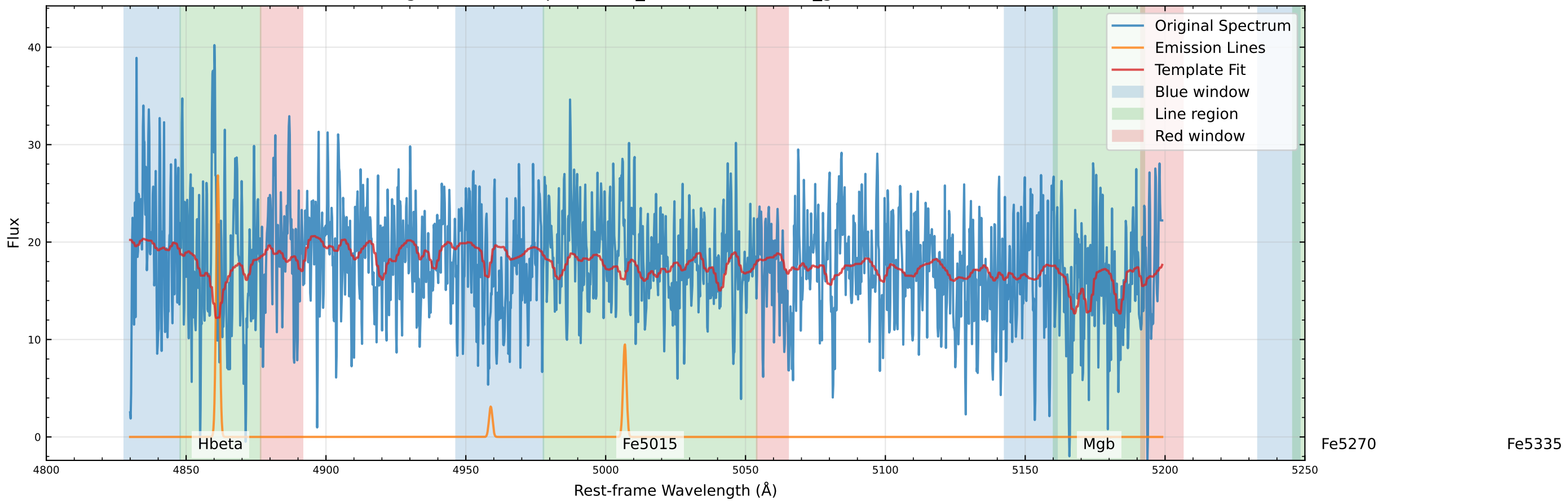
Original Data Comparison (v_star=-82.5 km/s, v_gas=-89.4 km/s)
