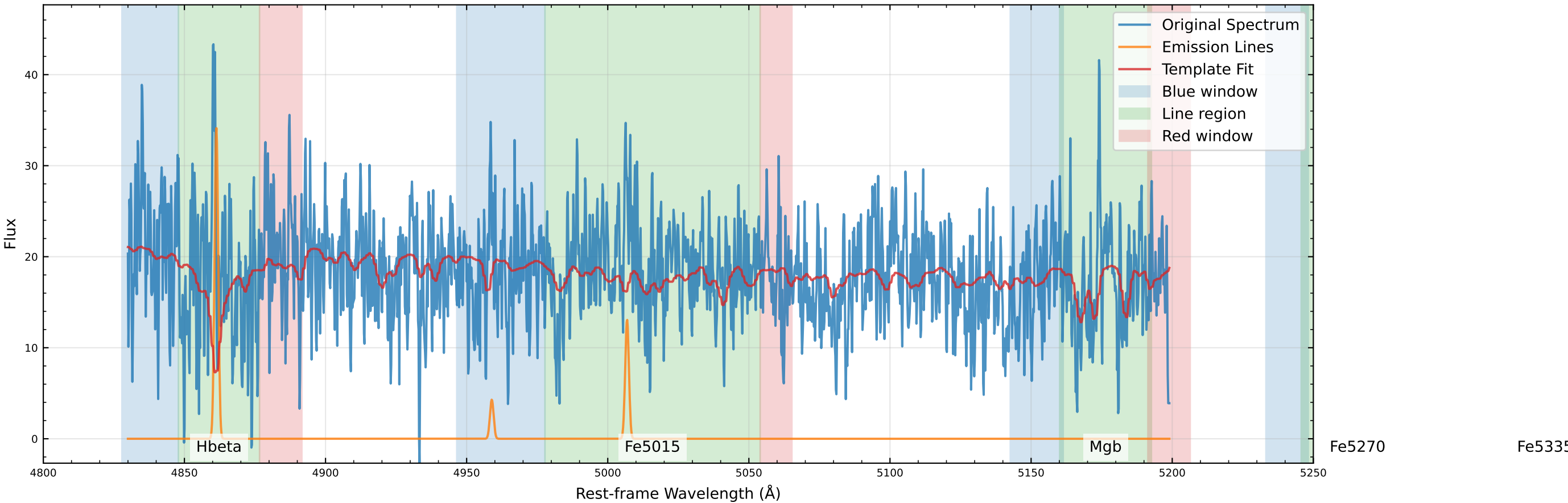
Original Data Comparison (v_star=-47.0 km/s, v_gas=-52.9 km/s)
