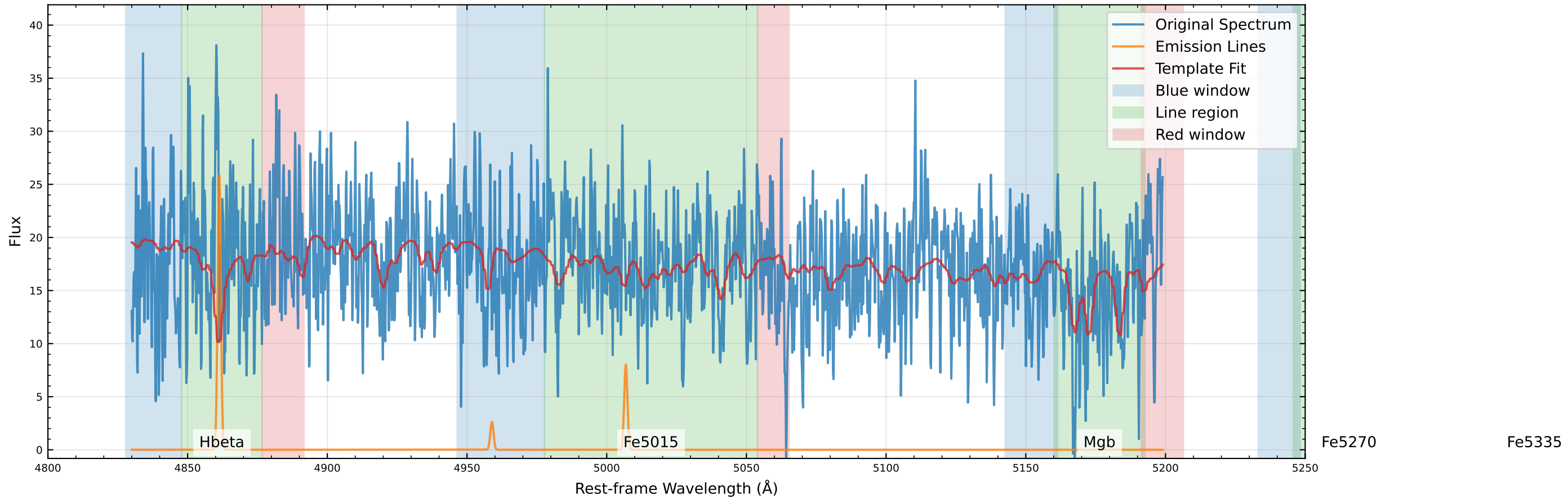
Original Data Comparison (v_star=-12.9 km/s, v_gas=-58.1 km/s)
